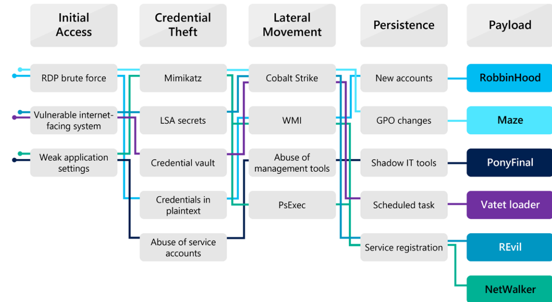
Ransomware operations attack pattern detail observed by Microsoft Threat Protection intelligence in early 2020. Payloads might vary, but mitigations apply across all varieties.
