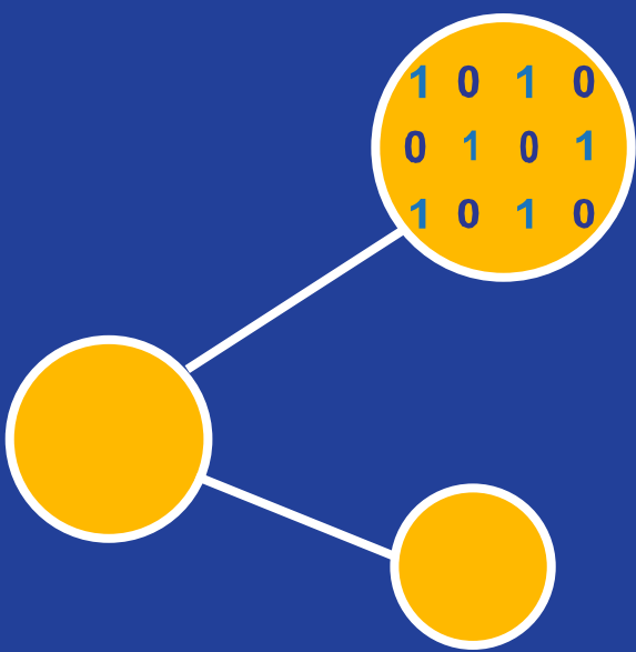
Big Data
